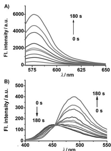
Figure 1. The emission spectra of probe 1 ( 0.6\ \mu\text{M} in 25\ \text{mM} sodium phosphate buffer, pH 7.0, containing 10% DMF) prior to exposure to visible light, and after increasing duration of illumination with visible light. A) Emission changes in the rosamine emission region with \lambda_{\text{ex}} = 554\ \text{nm} (ex = excitation); B) Emission changes in the coumarin emission region with \lambda_{\text{ex}} = 396\ \text{nm} . The duration of light exposure is in seconds.
